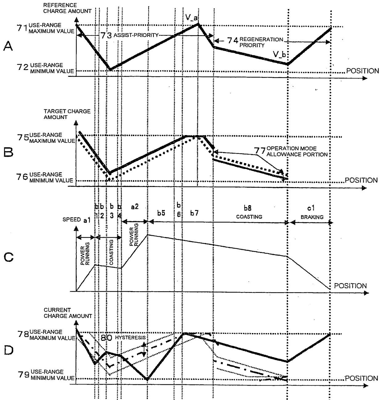
DIAGRAM ILLUSTRATING ANOTHER SPECIFIC CONTROL EXAMPLE IN RUNNING
