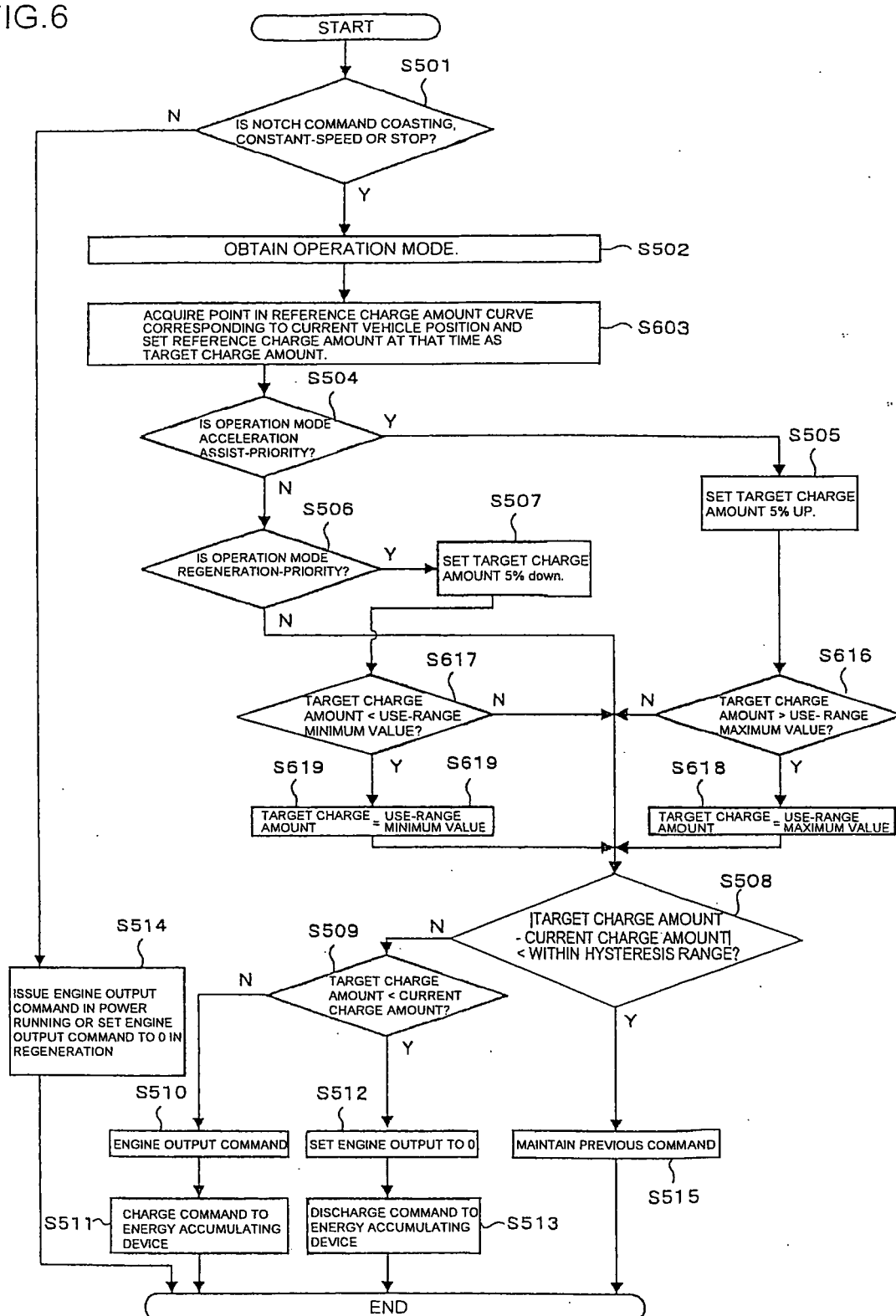
PROCESSING FLOWCHART OF ANOTHER TRAIN CONTROL DEVICE
