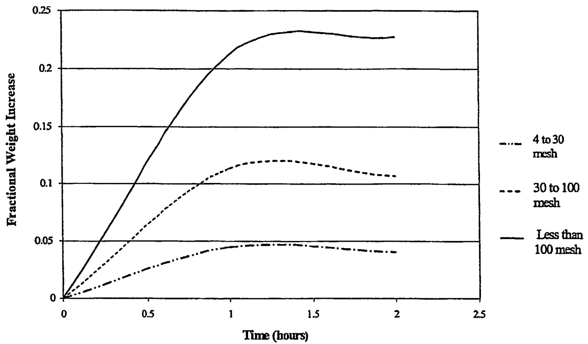
Figure 1. Effect of particle size on fractional weight gain due to TE oxidation in smelter matte.
