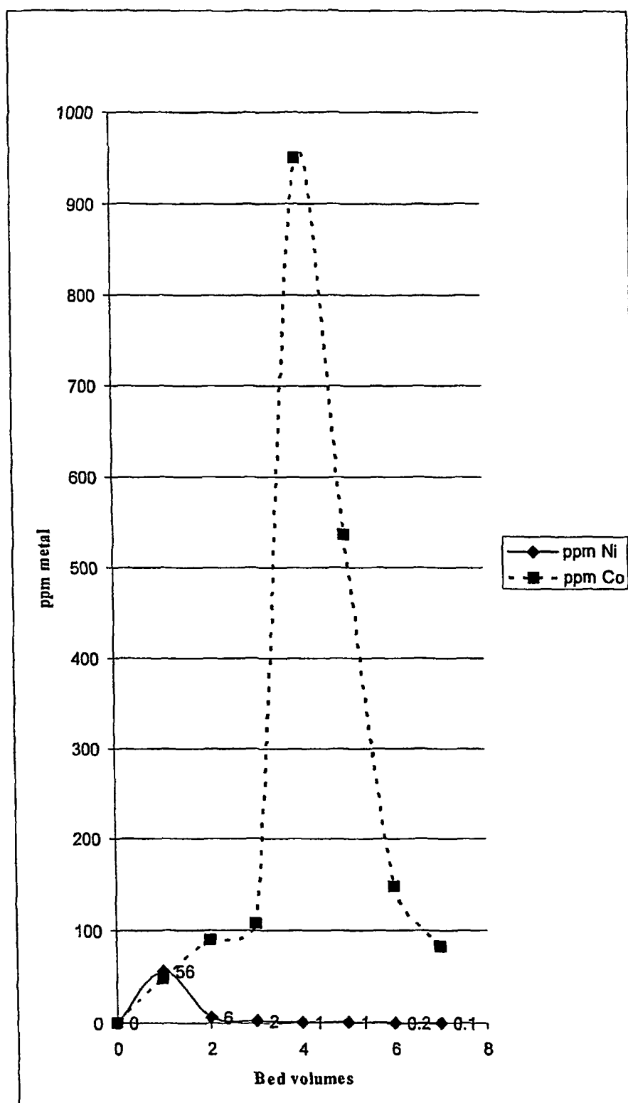
Figure 3. Removal of Ni and purification of Co in 12N HCl.
