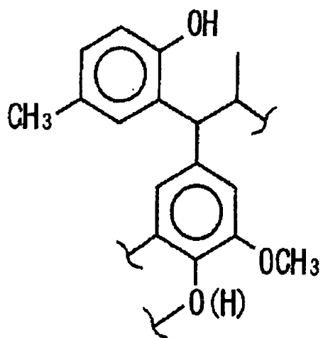
ortho-position binding unit
