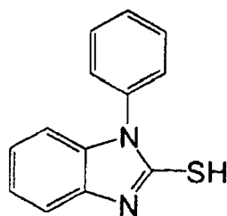
Additive (C - 1)
