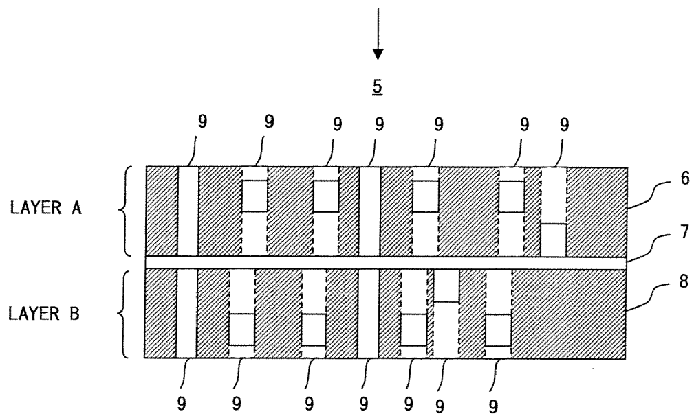
THERMAL ANALYSIS MODEL ACCORDING TO PRESENT INVENTION
