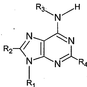
Figure 6a, Adenine, A
