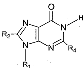
Figure 6f, Inosine, I
