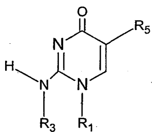
Figure 6p, isoCytosine, isoC
