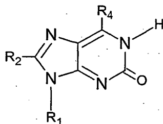
Figure 6o, 2-oxoPurine, Pu-2o
