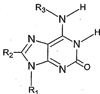
Figure 6m, isoGuanine, isoG
