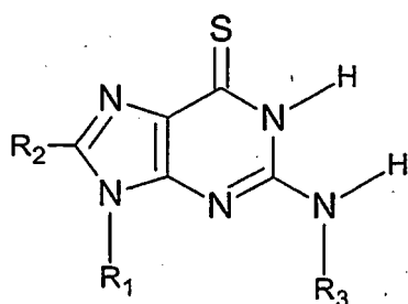
Figure 6e, ThioGuanine, Gs
