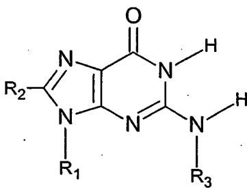
Figure 6d, Guanine, G
