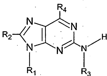
Figure 6b, isoAdenine, isoA
