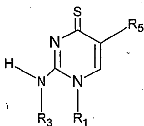
Figure 6q, isothioCytosine, isoCs
