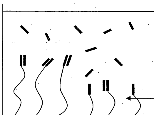
Figure 5B: Capture fast relative to diffusion
