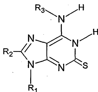
Figure 6n, isothioGuanine, isoGs
