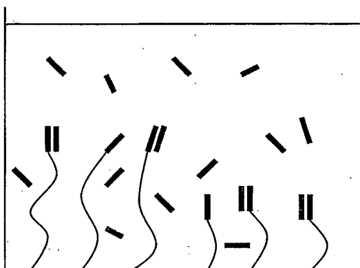
Figure 5A: Capture slow relative to diffusion
