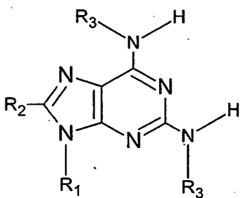
Figure 6c, Diaminopurine, D
