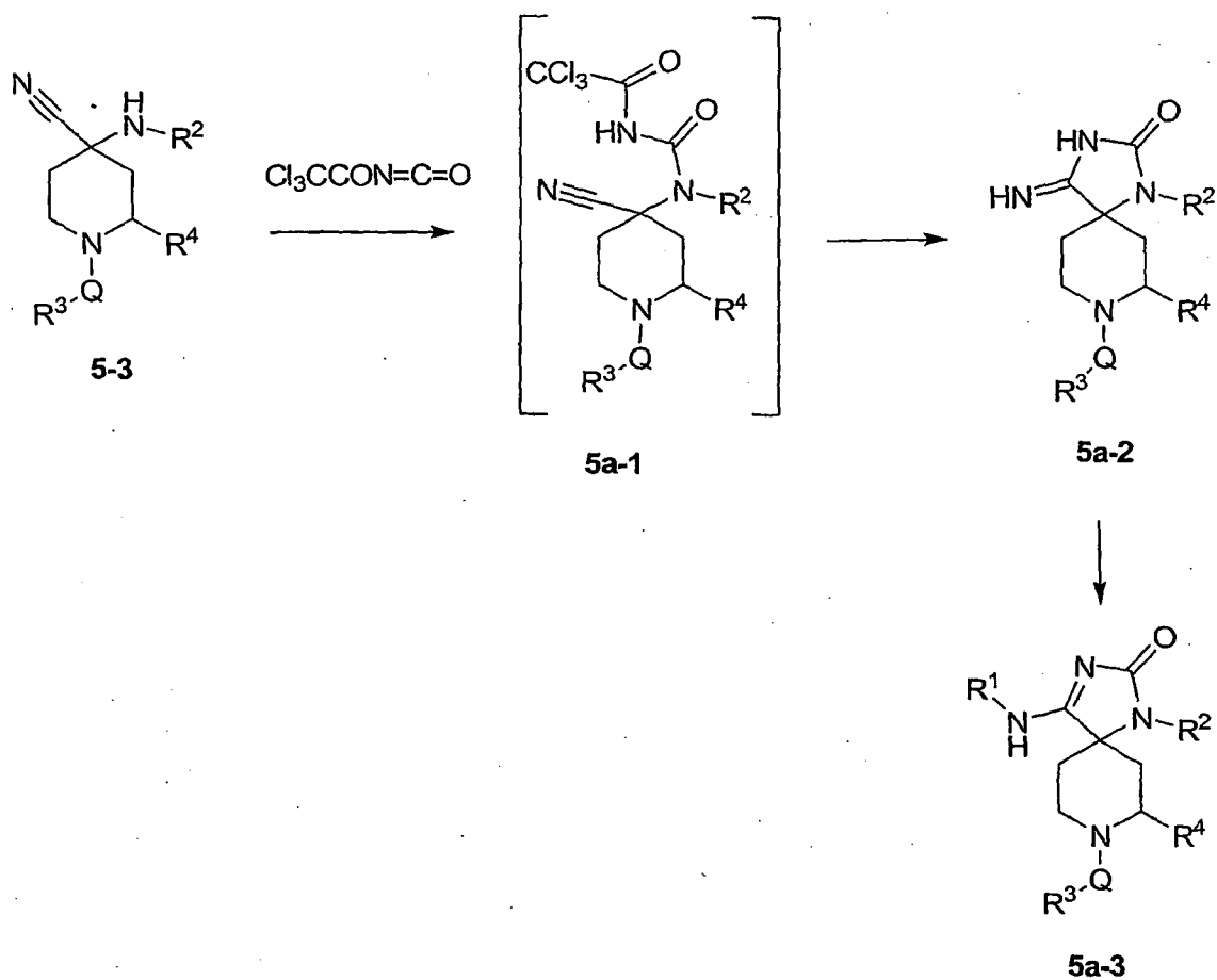
General Scheme 5a
