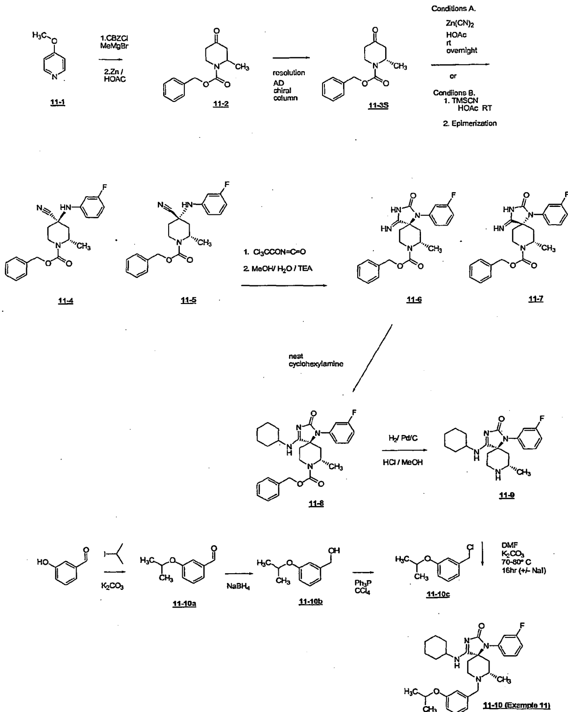
Scheme for Example 11 (Adapted from General Scheme 7)
