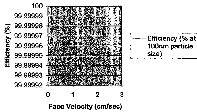
Filter Efficiency vs. Face Velocity
