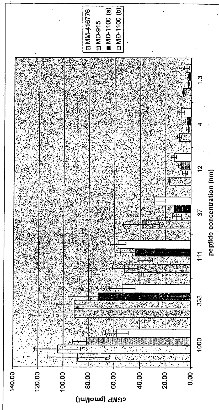
Figure 2. Chemically synthesized peptides in the Intestinal GC-C Receptor Activity Assay
