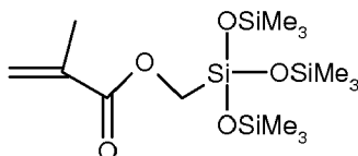
methacryloxymethyltris(trimethylsiloxy)silane
