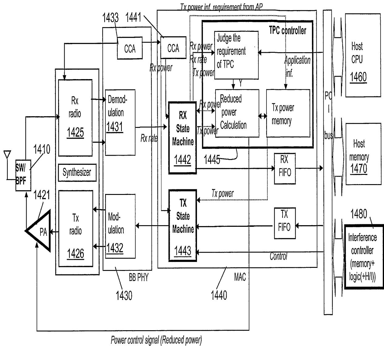
Figure 14: Block Diagram of STA for TPC
