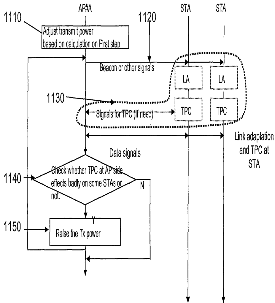
Figure 11: Flow Chart of the Second Step of TPC Method of AP (iv)
