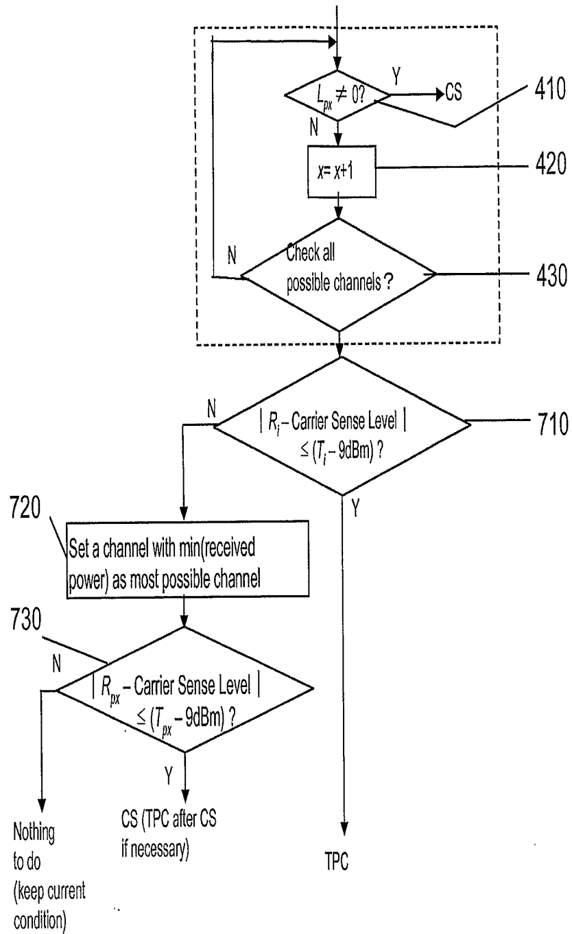
Figure 7: Selection Flow with Policy 2 ((i)-policy2-a)
