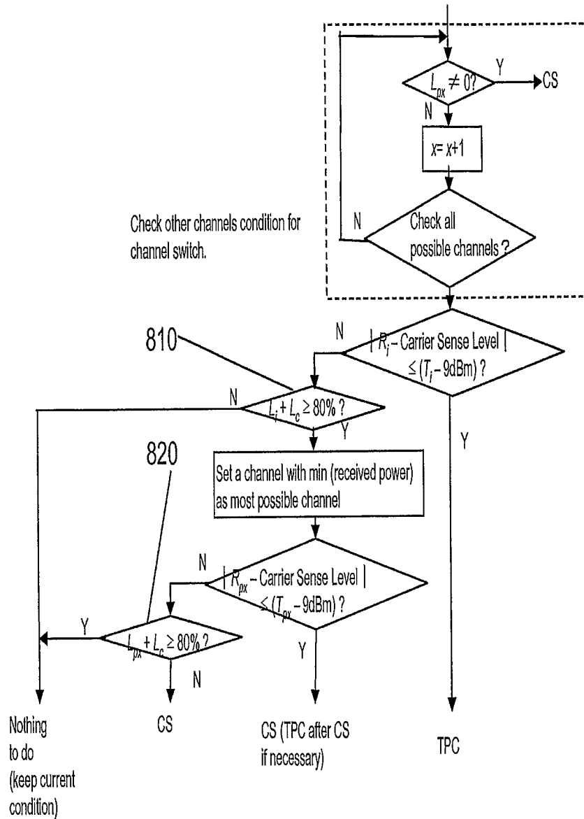
Figure 8: Advanced Selection Flow with Policy 2 ((i)-policy2-b)
