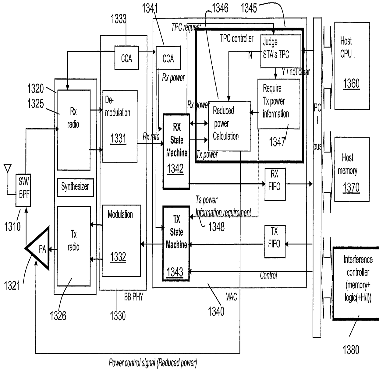
Figure 13: Block Diagram of AP for TPC
