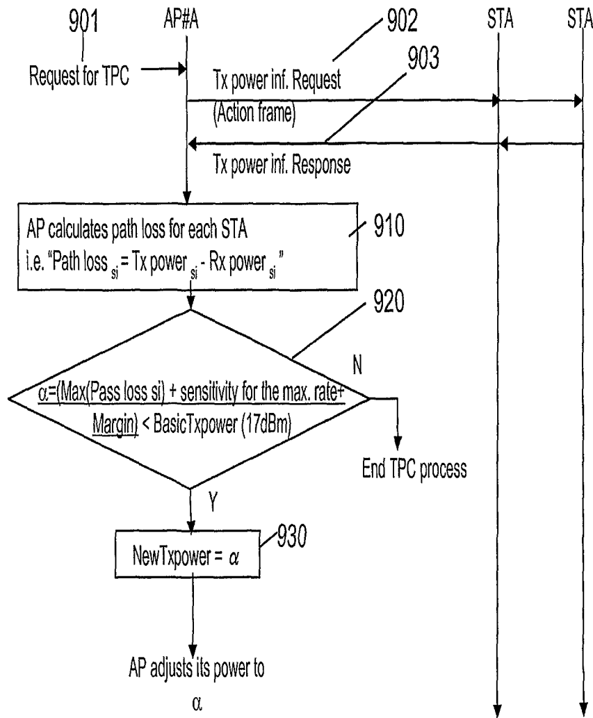
Figure 9: Flow Chart (First Step of TPC Method of AP, (iii)-a)
