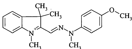
Cation of Basic Yellow 28
