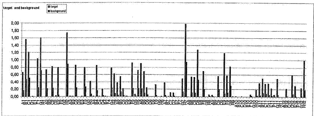
Fig. 9: Exemplary hit-ELISA showing variants of the SPA10 library versus TNF \alpha (red) and BSA (blue) as a background.
