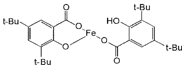
Aromatic oxycarboxylic acid metal compound 1
