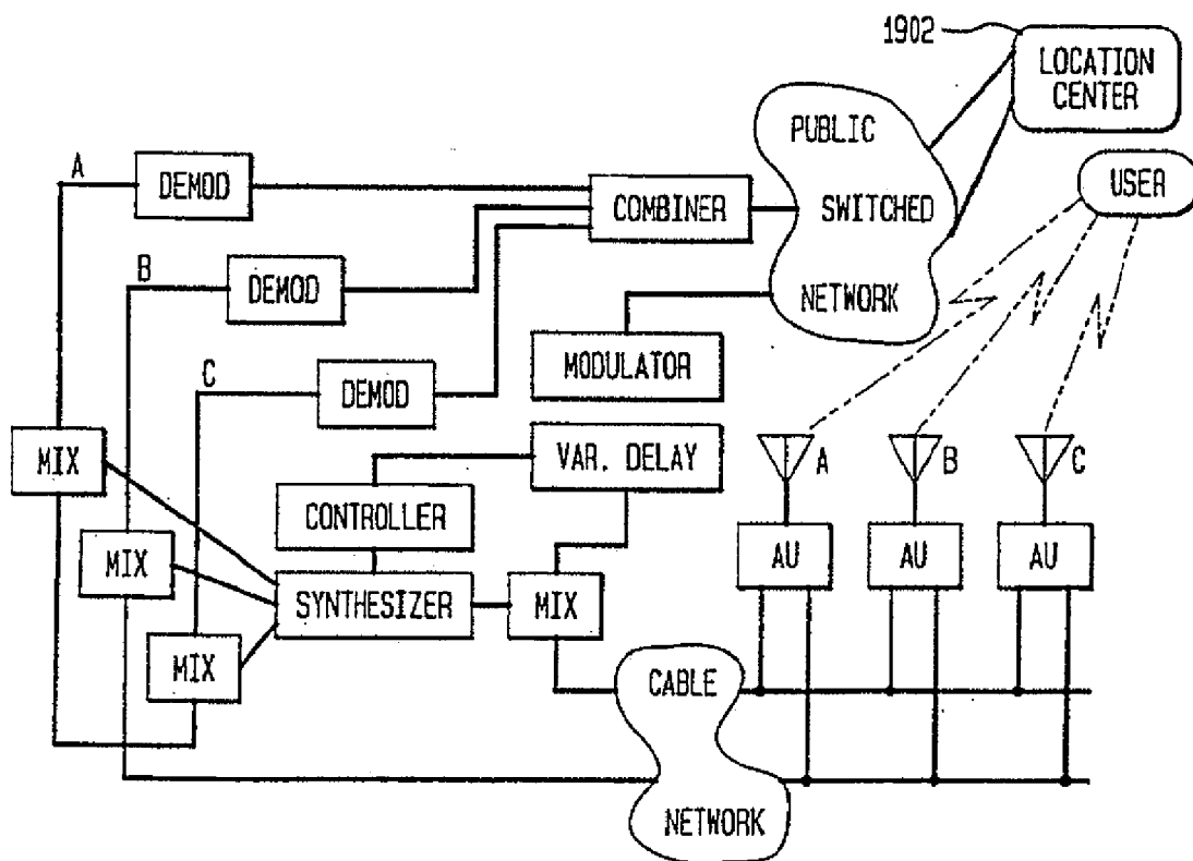
FIG. 19 LOCATION CENTER EXTERNAL TO COMMUNICATION SYSTEM
