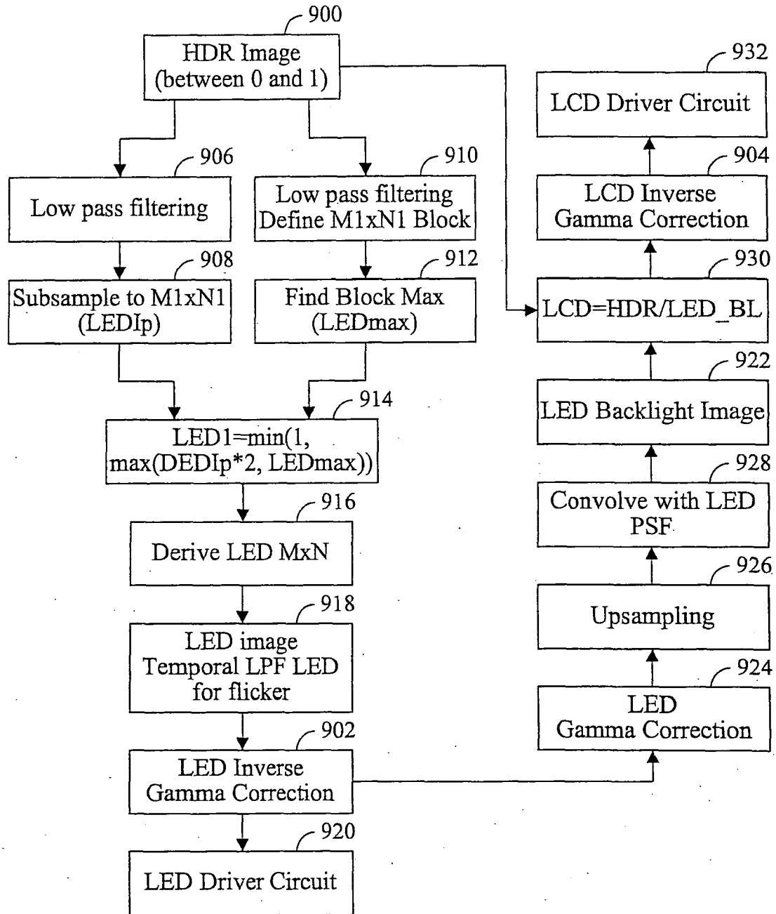
Flow chart of deriving LED and LCD driving values for HDR display
