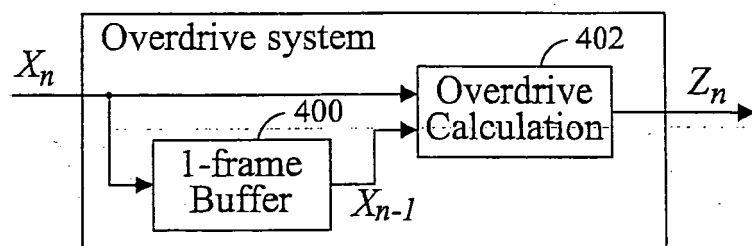
The one-frame buffer non-recursive overdrive model
