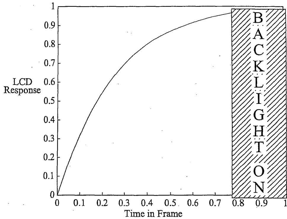
Flashing backlight scheme to reduce the motion blur
