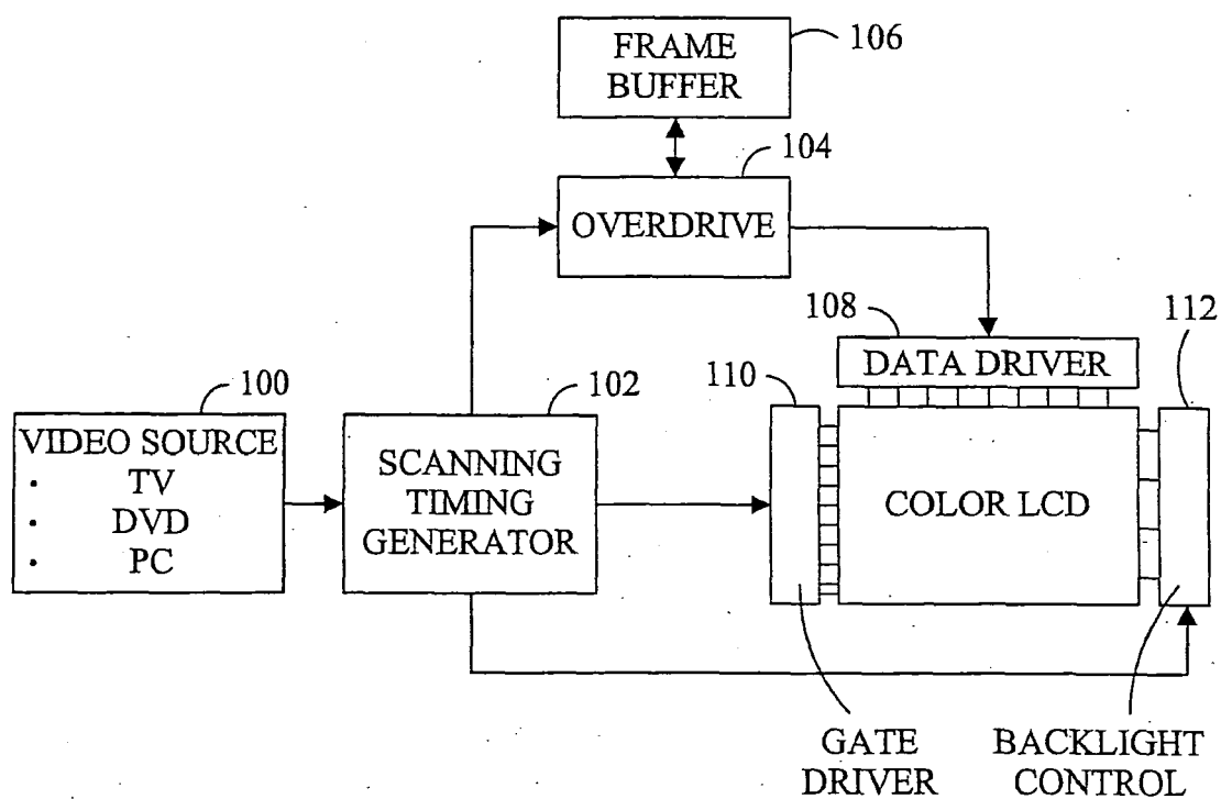
LCD system configuration
