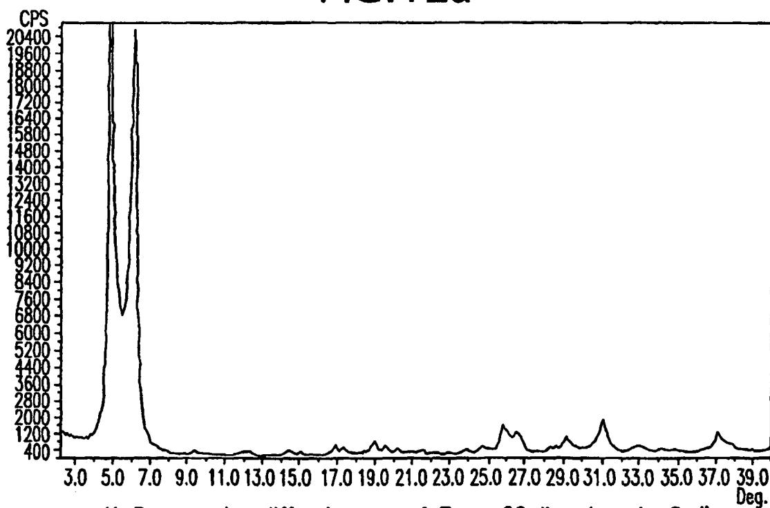
X-Ray powder diffractogram of Form Q2 Ibandronate Sodium
