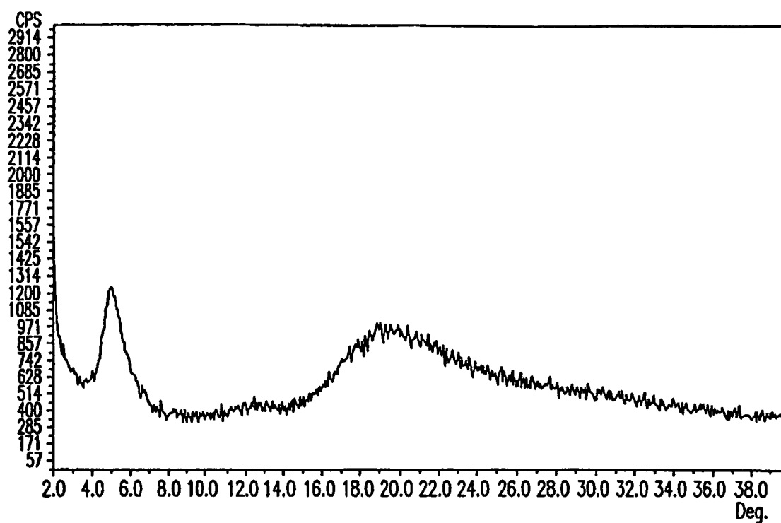
X-Ray powder diffractogram of amorphous Ibandronate Sodium
