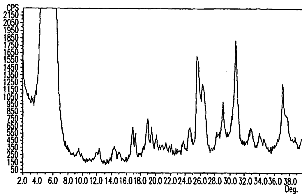
X-Ray powder diffractogram of Form Q2 Ibandronate Sodium FIG.13a
