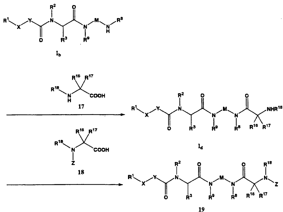
Scheme 8
