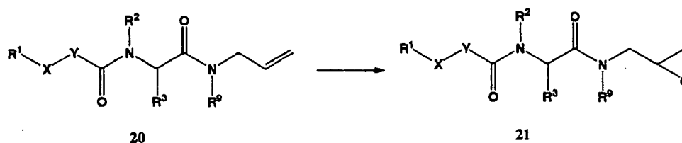
Scheme 10
