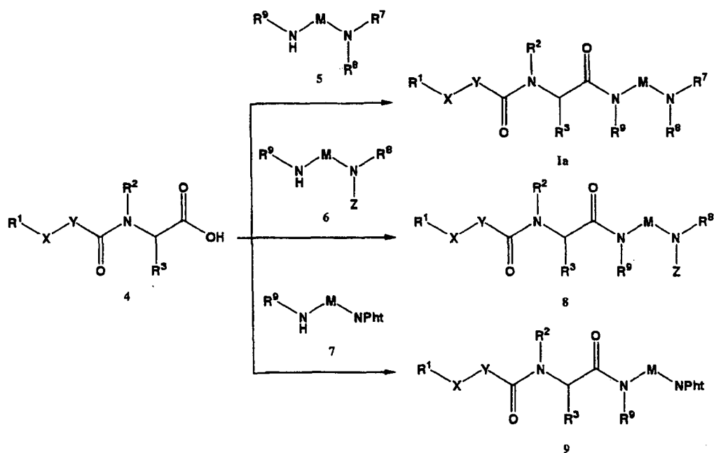
Scheme 3
