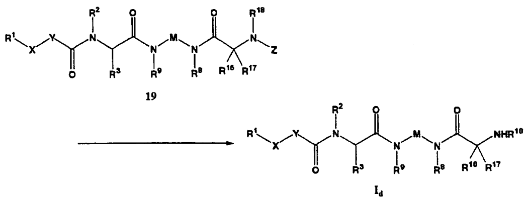
Scheme 9
