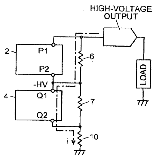
(b) NEGATIVE VOLTAGE OUTPUT
