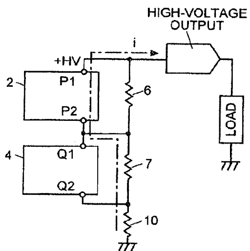
(a) POSITIVE VOLTAGE OUTPUT
