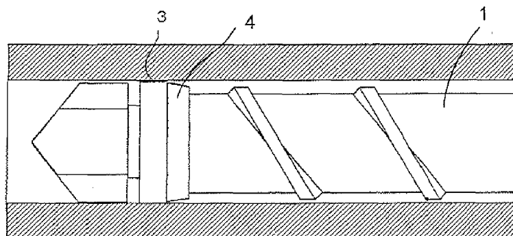
FIG. 4D STATE WHERE SCREW MOVES FORWARD IN INJECTION/HOLD PRESSURE STEP
