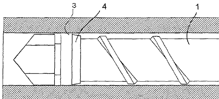
FIG. 3D WHEN THE SCREW REACHES INJECTION/HOLD PRESSURE SWITCHING POSITION
