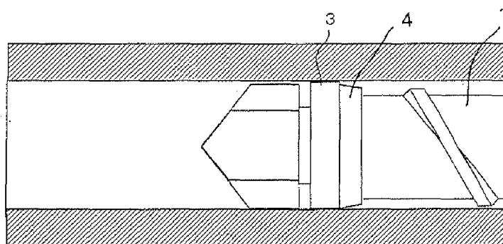
FIG. 4C WHEN SCREW RETRACTS TO INJECTION STARTING POSITION
