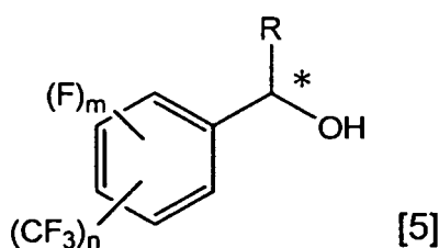
[Chemical Formula 33]
