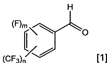
[Chemical Formula 29]
