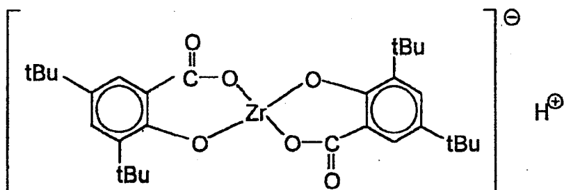
Zirconium complex (12):
