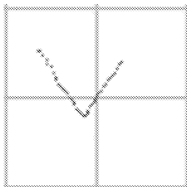
(f) PARABOLIC INTERPOLATION METHOD APPLIED
