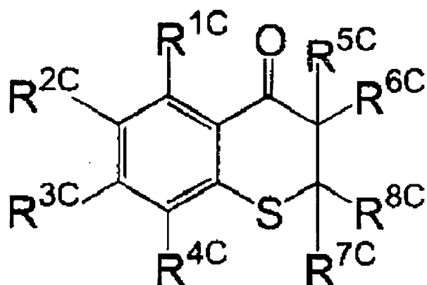
Formula (I-C)
