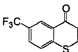
(I-7)
