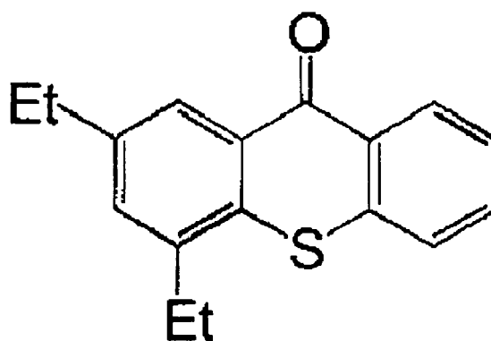
(2,4-diethylthioxanthone)
