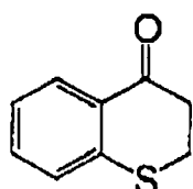
(I-1)
