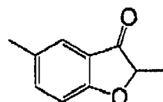
(I-100)
