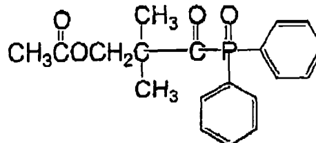
(P-8)
