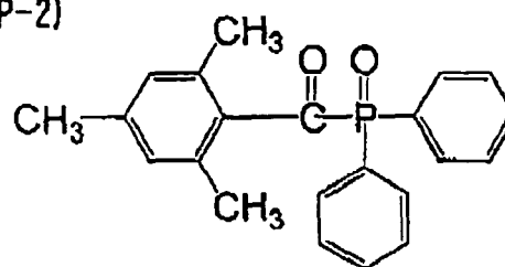
(P-2)
