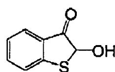
(I-79)
