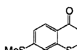
(I-12)
