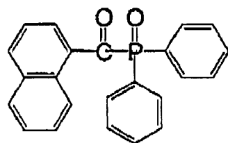
(P-15)
