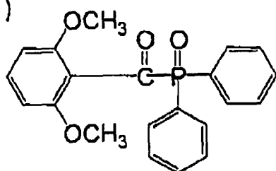
(P-2)
