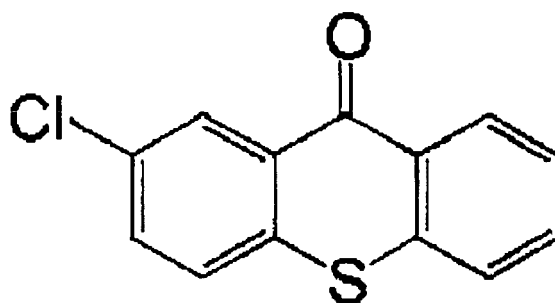
(2-Chlorothioxanthone)
