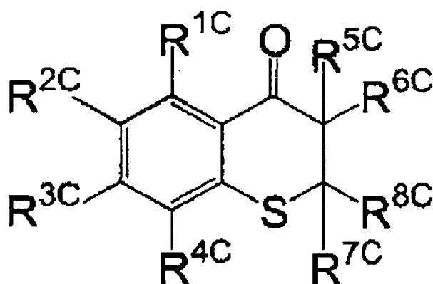
Formula (I-C)
