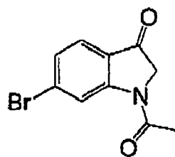
(I-123)
