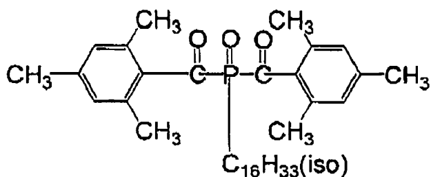
(P-24)
