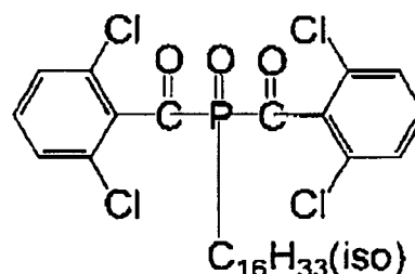
(P-26)
