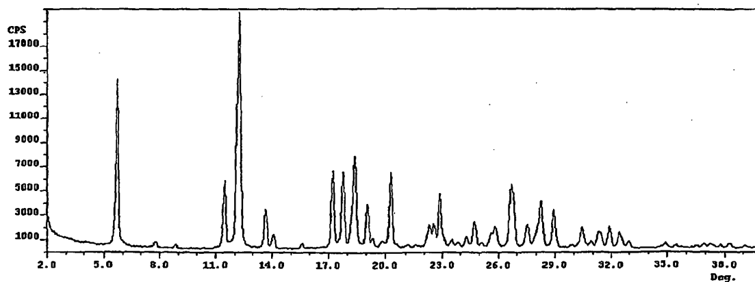
Fig.2: An X-ray powder diffraction pattern of crystalline pemetrexed diacid characterized by an X-ray powder diffraction pattern with peaks at about 5.7, 12.2, 17.2 and 18.4 degrees two-theta \pm 0.2 degrees two-theta.
