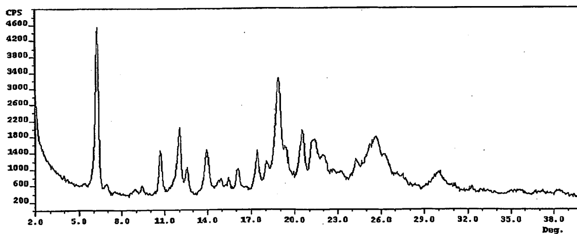
Fig.4: An X-ray powder diffraction pattern of crystalline pemetrexed diacid characterized by an X-ray powder diffraction pattern with peaks at about 6.2, 10.7, 12.0 and 18.9 degrees two-theta \pm 0.2 degrees two-theta.
