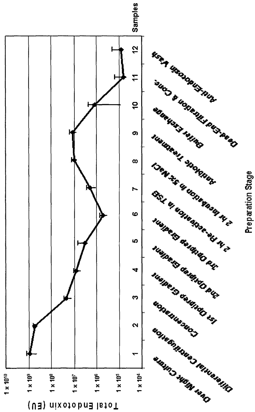
Figure 6C Total endotoxin (EU) at each stage of the minicell purification procedure
