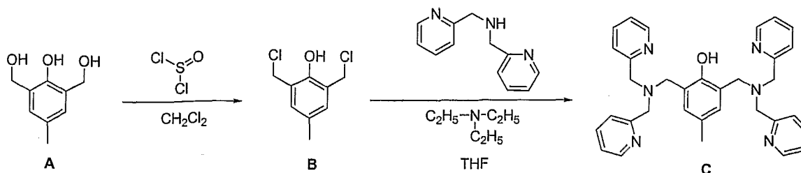
Scheme 1. Synthesis of h-BPMP (2,6-Bis(bis(2-pyridylmethyl)aminomethyl)-4-methylphenol)
