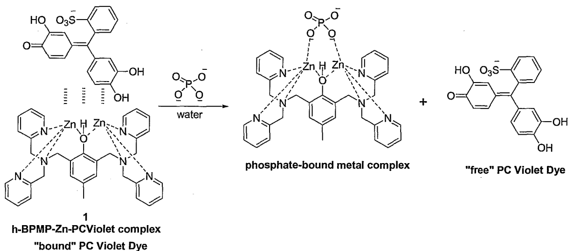
Scheme 2. Mechanism of sensing phosphate in an aqueous test sample as described in tests 2 and 3
