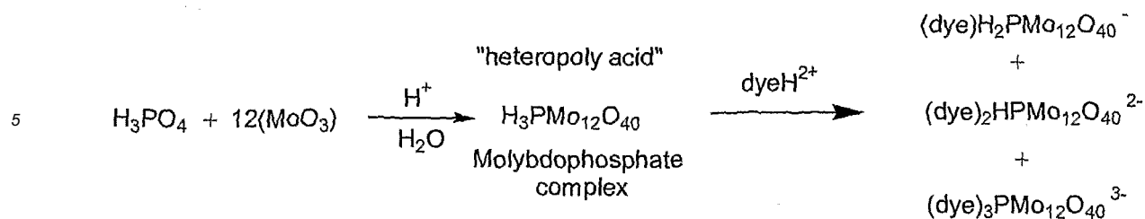
Scheme 3. Mechanism of sensing phosphate in an aqueous test sample as described in tests 4 to 14.
