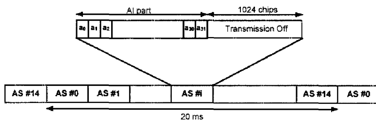
Figure 84: Structure of the AICH
