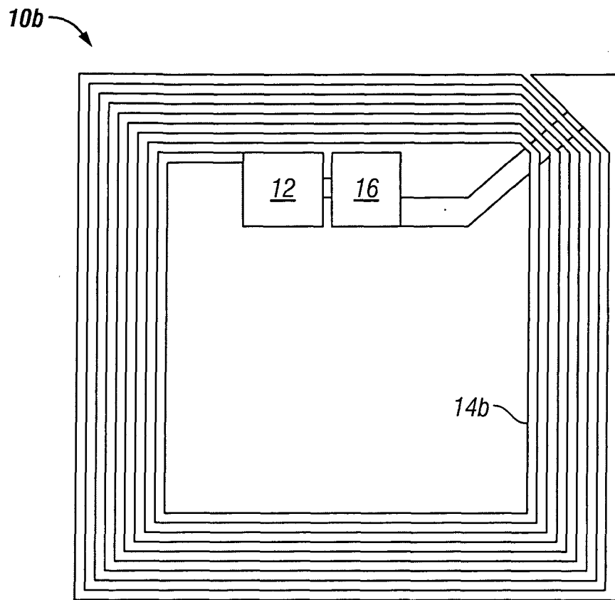
FIG. 3 (Prior Art)
