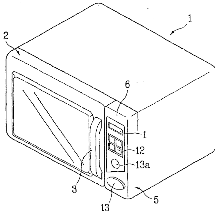
FIG.2 Related Art
