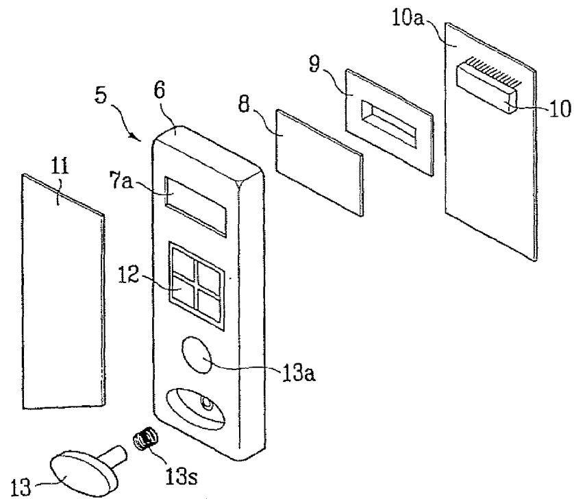
FIG.2 Related Art
