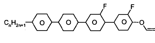
PPGU-n-OXF
