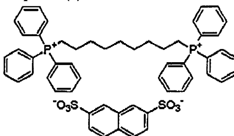
Phosphonium compound (1)
