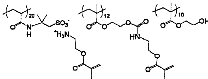
Undercoating compound (1)
