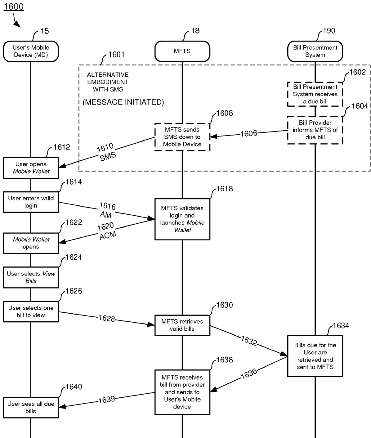
SEQUENCE DIAGRAM FOR VIEWING BILLS
