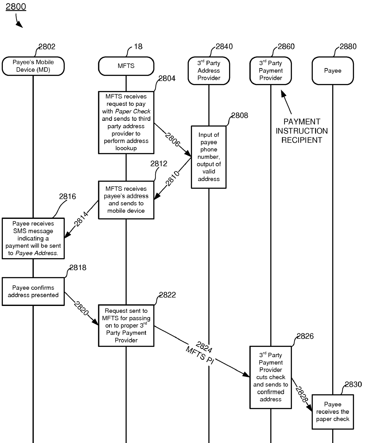
SEQUENCE DIAGRAM FOR PAYANYONE WITH PAPER CHECK FIG. 28
