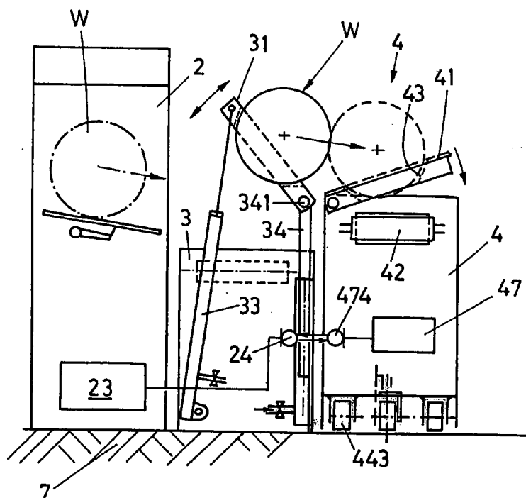
Fig.1 (prior art)
