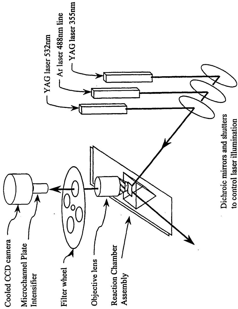
FIG. 7 Setup for DNAS using TIRFM
