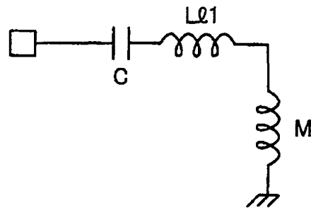
FIG. 8B LOAD-CONNECTED
