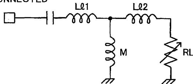
FIG. 8B LOAD-CONNECTED
