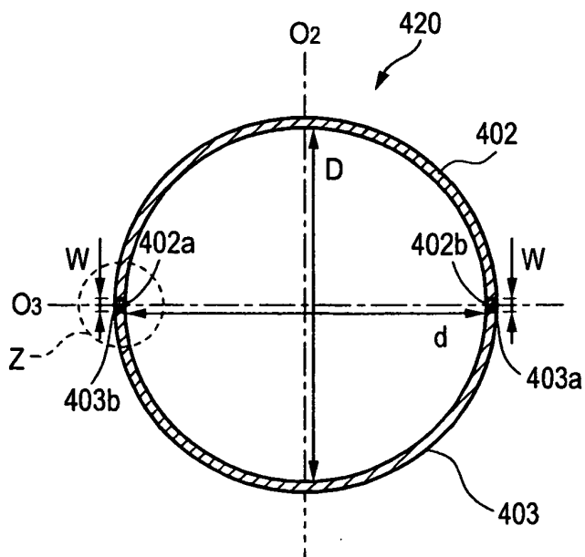
X-X SECTIONAL VIEW
