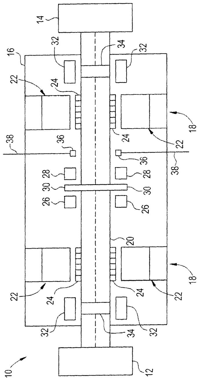
FIG. 1 PRIOR ART
