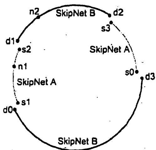
Figure 14. Two partitioned SkipNets to be merged.
