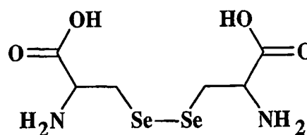
Selenocystine
