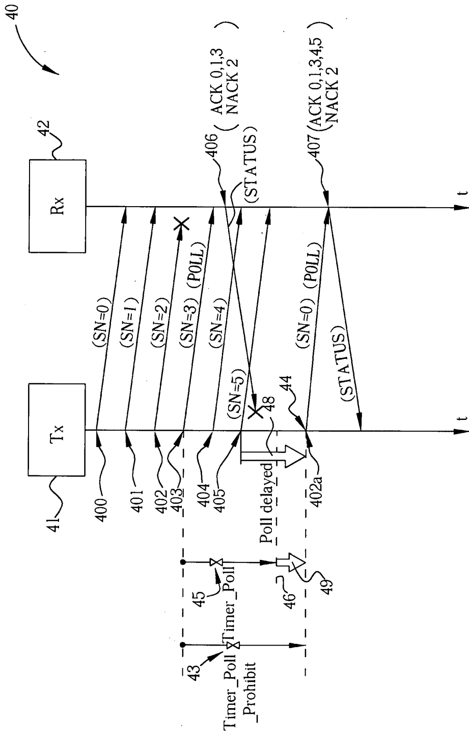
FIG. 5 PRIOR ART
