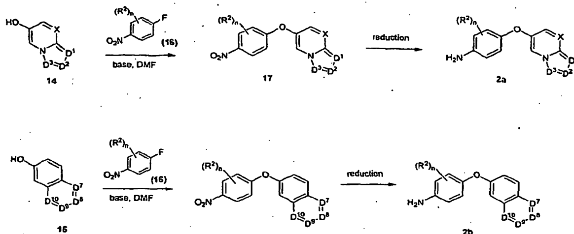
Scheme 5
