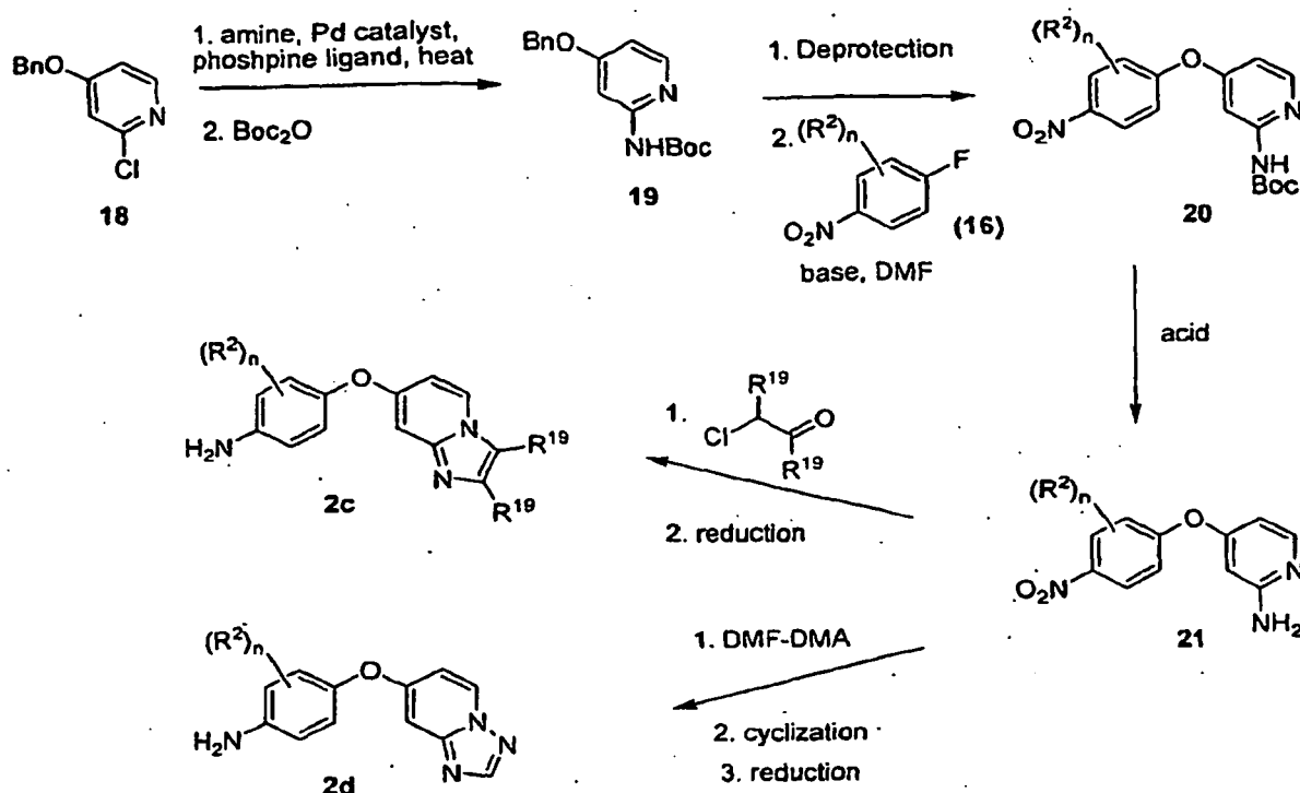
Scheme 8
