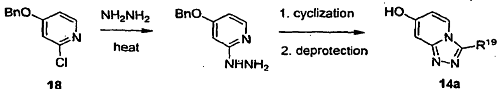
Scheme 6
