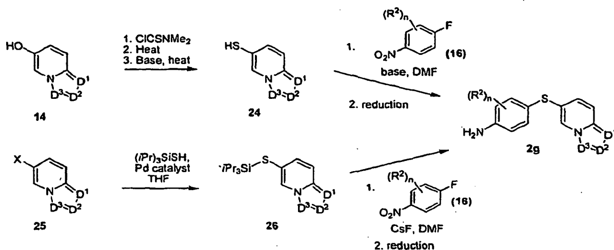
Scheme 10
