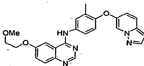
N-(4-(H-pyrazolo[1,5-a]pyridin-6-yloxy)-3-methylphenyl)-6-(2-methoxyethoxy)quinazolin-4-amine hydrochloride
