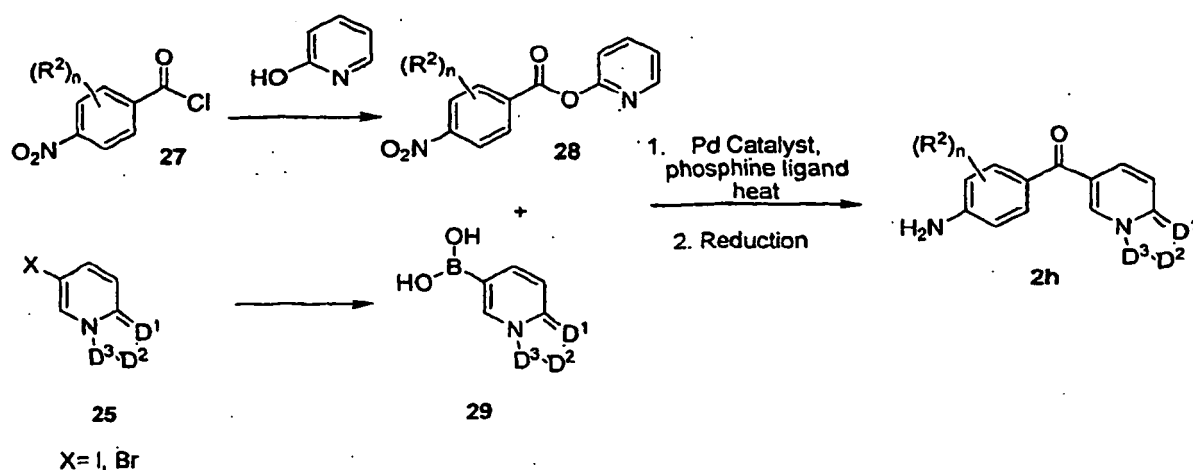
Scheme 11
