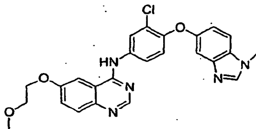
N-(3-chloro-4-(1-methyl-1H-benzo[d]imidazol-5-yloxy)phenyl)-6-(2-methoxyethoxy)quinazolin-4-amine
