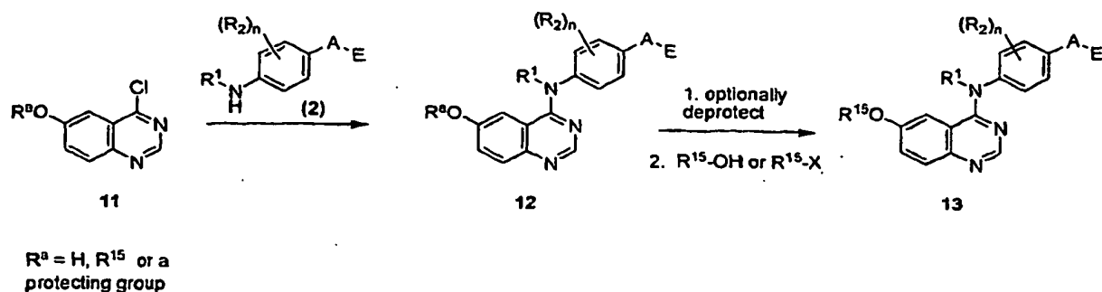
Scheme 4
