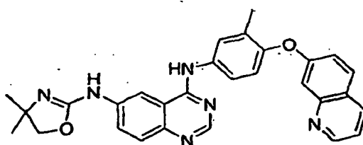
N6-(4,4-dimethyl-4,5-dihydrooxazol-2-yl)-N4-(3-methyl-4-(quinolin-7-yloxyphenyl)quinazoline-4,6-diamine
