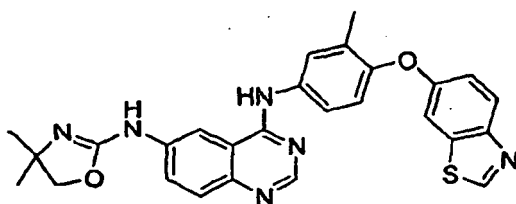
N4-(4-(benzo[d]thiazol-6-yloxy)-3-methylphenyl)N6-(4,4-dimethyl-4,5-dihydrooxazol-2-yl)quinazoline-4,6-diamine
