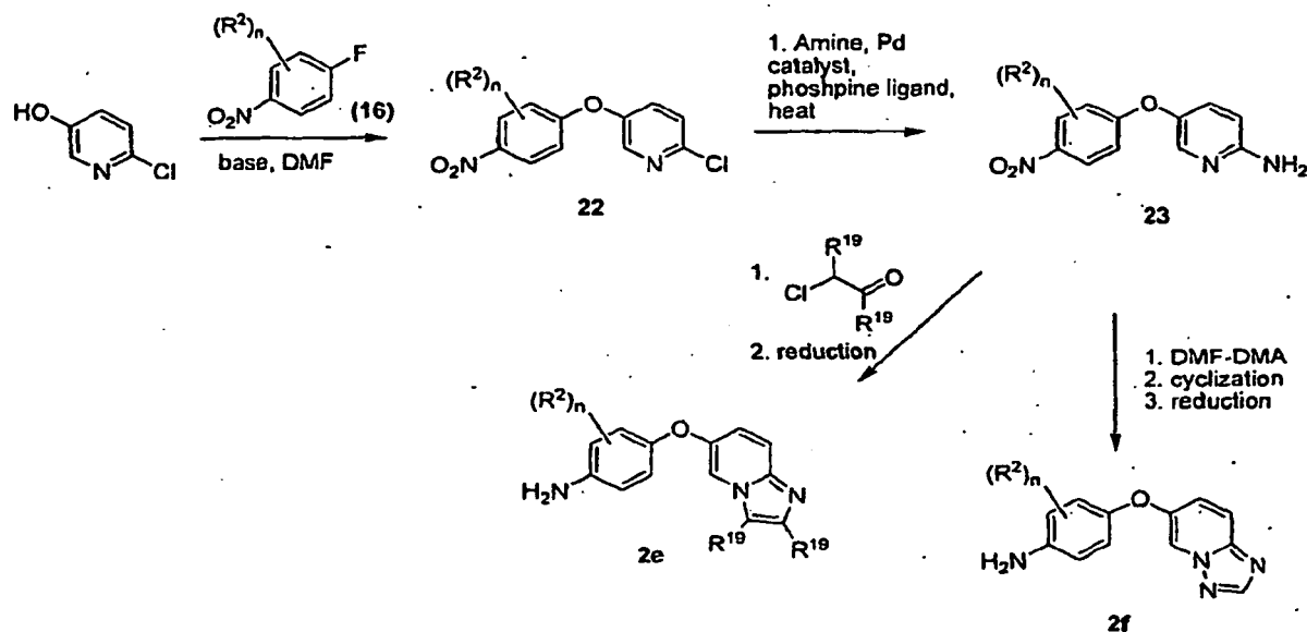
Scheme 9
