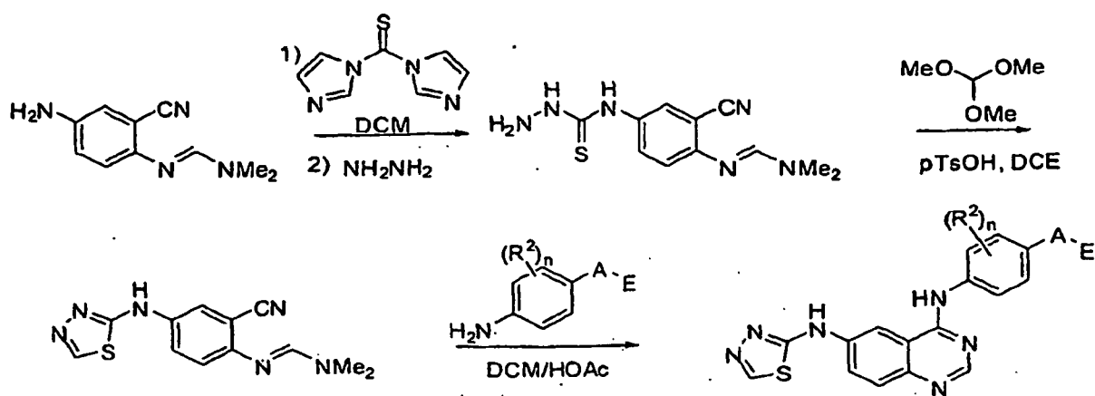
Scheme 13
