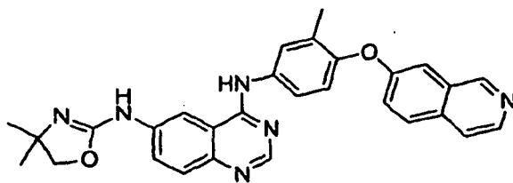
N6-(4,4-dimethyl-4,5-dihydrooxazol-2-yl)-N4-(4-(isoquinolin-7-yloxy)-3-methylphenyl)quinazoline-4,6-diamine
