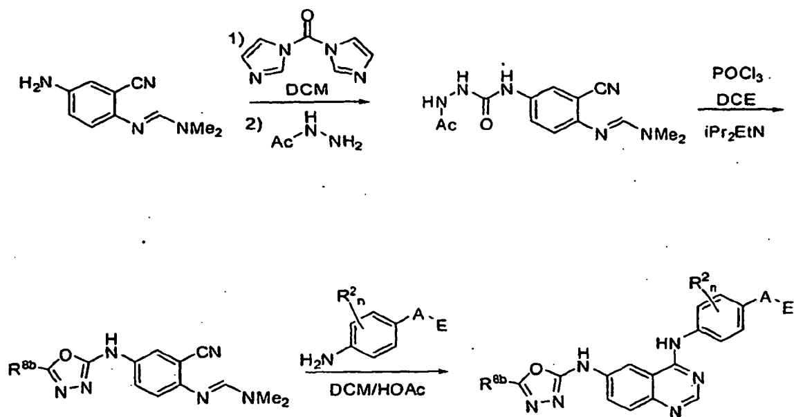
Scheme 12
