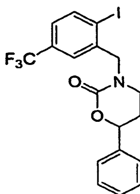
3-[2-iodo-5-(trifluoromethyl)benzyl]-6-phenyl-1,3-oxazinan-2-one
