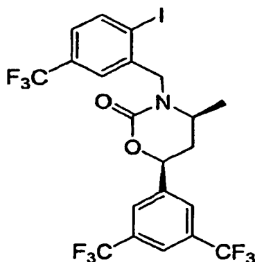
(4S,6S)-6-[3,5-bis(trifluoromethyl)phenyl]-3-[2-iodo-5-(trifluoromethyl)benzyl]-4-methyl-1,3-oxazinan-2-one
