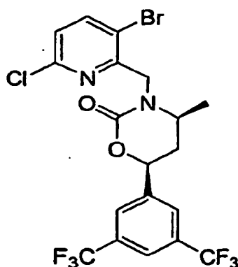
(4S, 6S)-6-[3,5-bis(trifluoromethyl)phenyl]-3-[(3-bromo-6-chloropyridin-2-yl)methyl]-4-methyl-1,3-oxazinan-2-one
