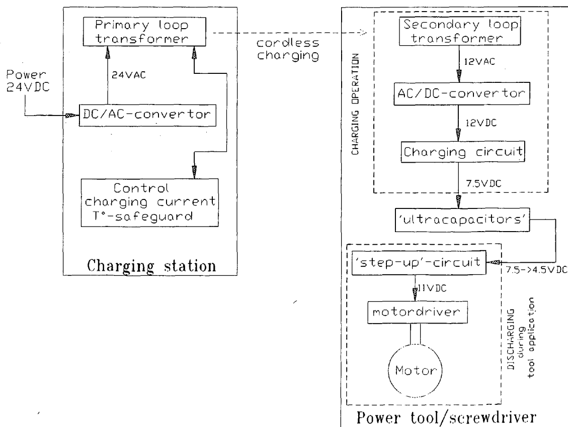
Figure 5 : Power scheme
