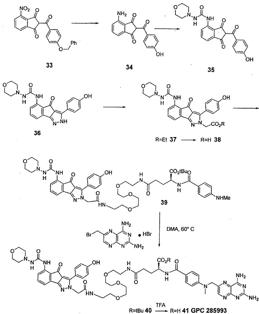
Scheme 6
