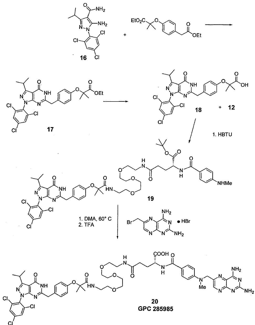
Scheme 3
