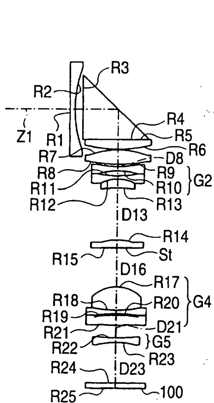
FIG. 7A EXAMPLE 7 (WIDE END)
