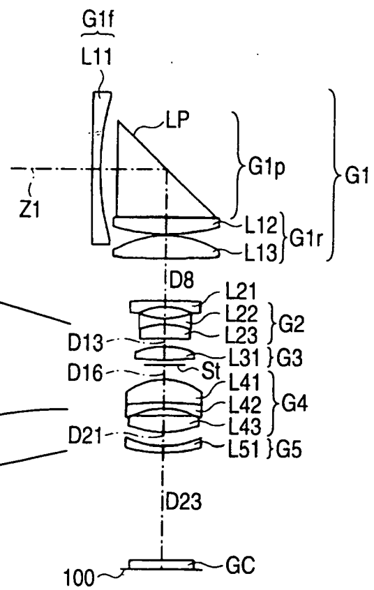
FIG. 2B EXAMPLE 2 (TELEPHOTO END)
