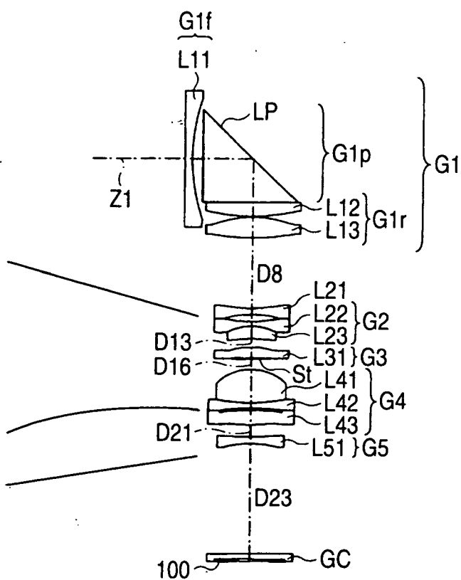
FIG. 7B EXAMPLE 7 (TELEPHOTO END)
