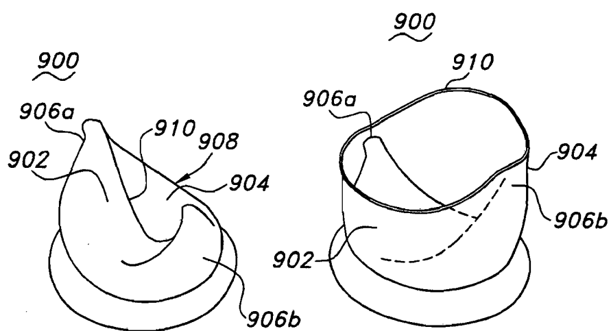
FIG 22 (PRIOR ART)
