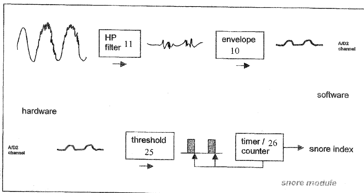
Figure 6 - snore algorithm module
