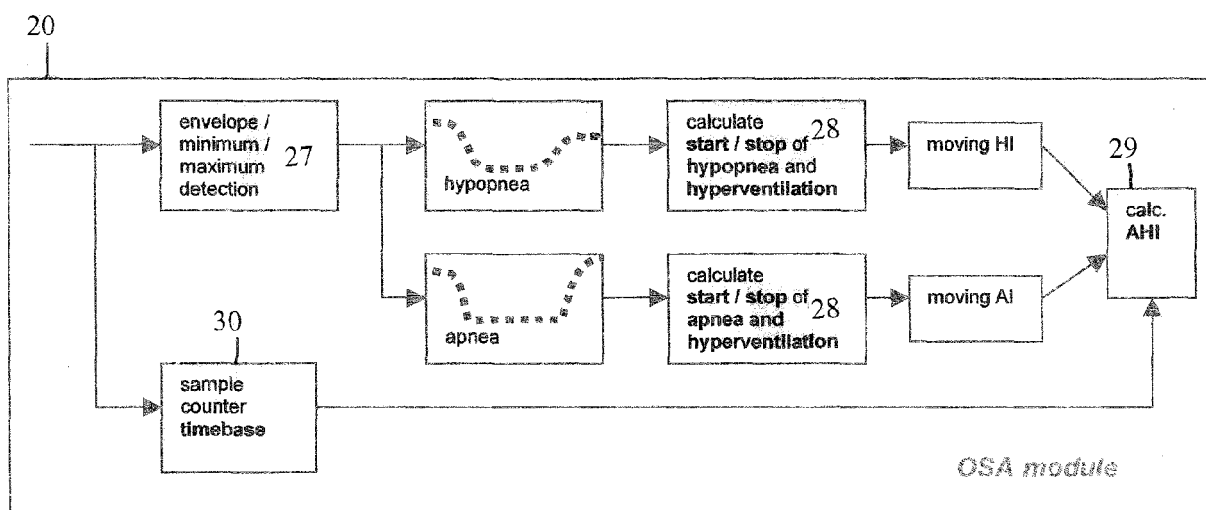
Figure 7 - OSA algorithm module
