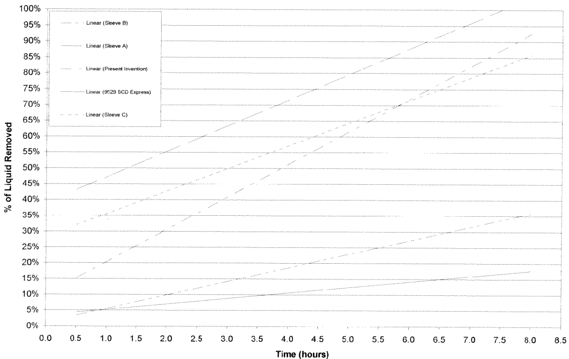
% of Liquid Evaporated vs. Time for Various Compression Sleeves
