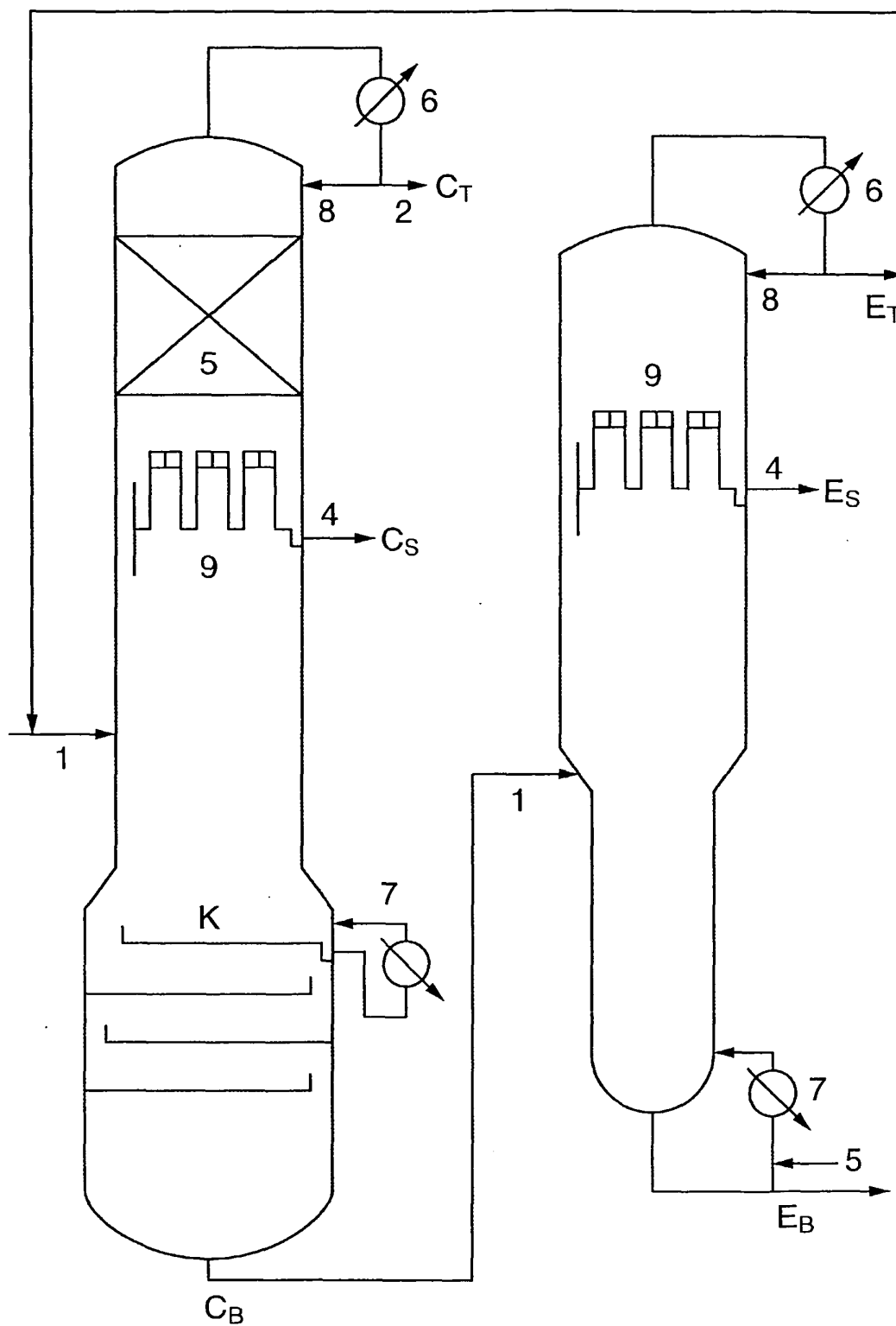
CONTINUOUS MULTI-STAGE DISTILLATION COLUMN C
